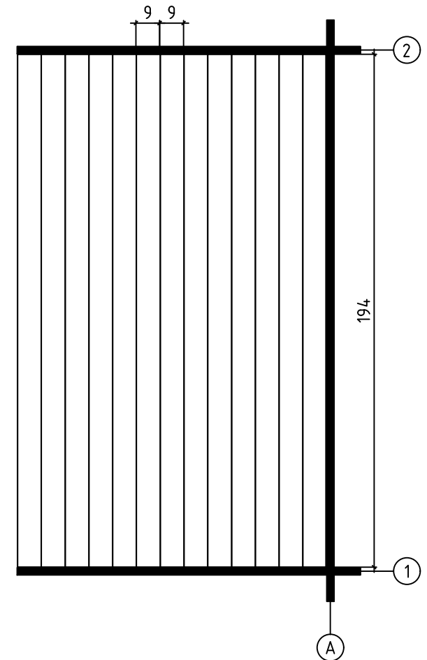
FLOOR BOARDS - FUSSBODENBRETTER - PLAN POSE PLANCHER
